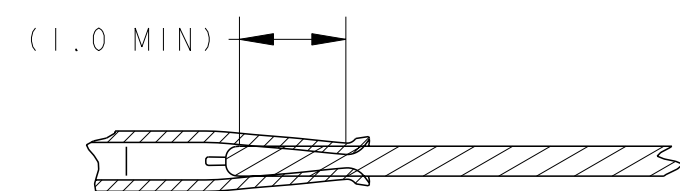
SOCKET CONTACT - CONTACT WIPE SCALE 10:1
