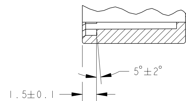
SECTION X-X ALL CODING RIBS
