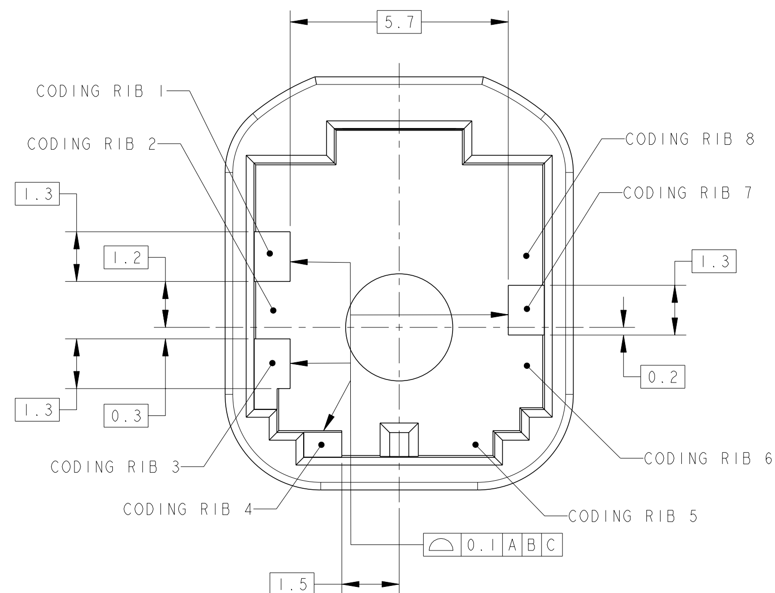
POLARIZATION CODING RIB LOCATIONS SCALE 10:1 ALL CODING RIBS (CODE E SHOWN FOR REFERENCE ONLY SEE POLARIZATION CODING TABLE)
