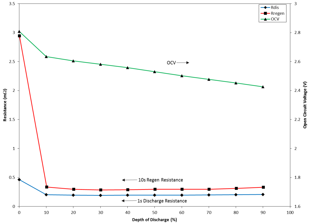
Figure 9. Open-circuit voltage and pulse resistances versus capacity removed.
