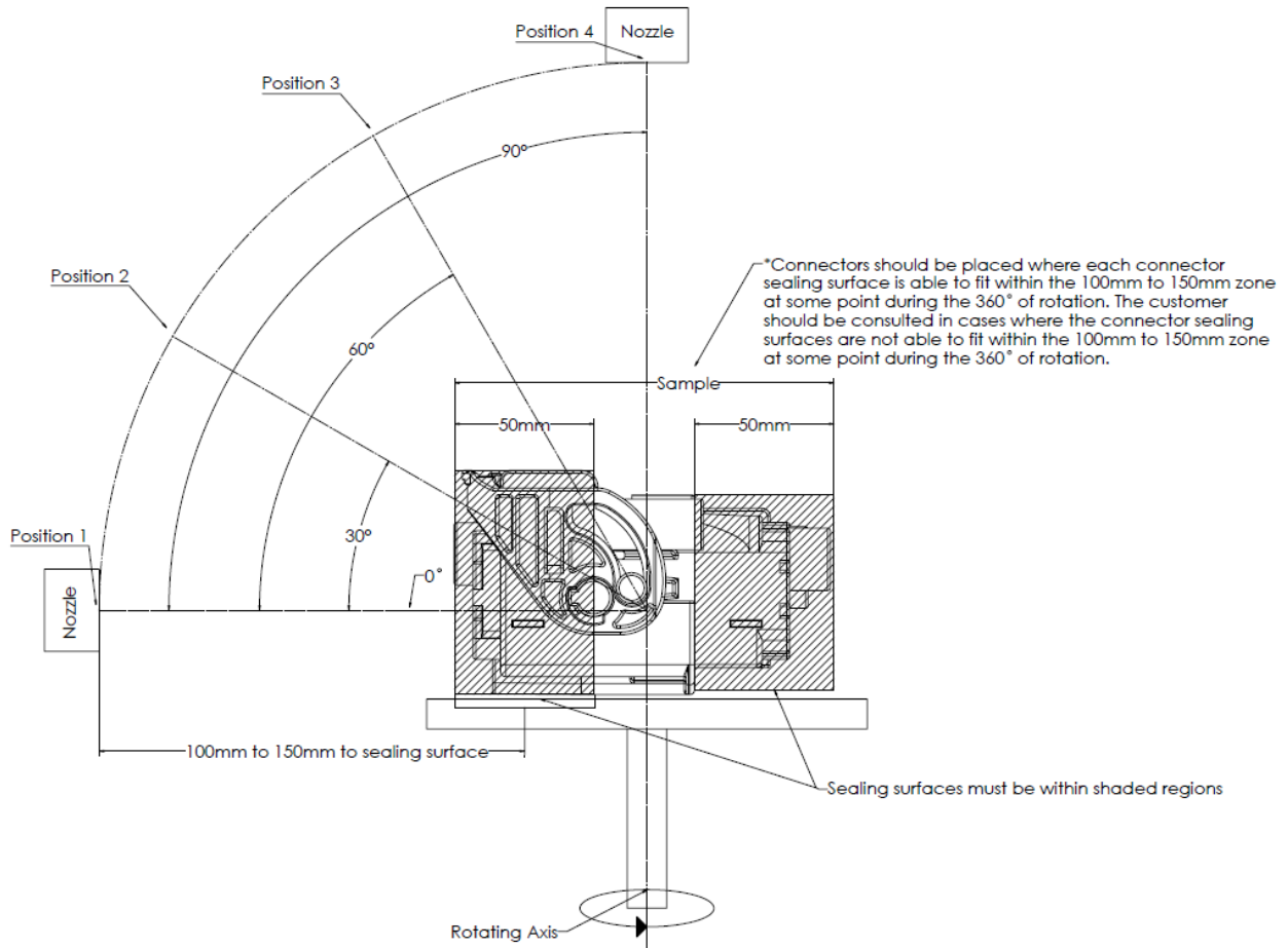
NEW FIGURE 5.6.7.3-2 DETAIL ON SPRAY NOZZLE PLACEMENT FOR LARGE CONNECTORS
