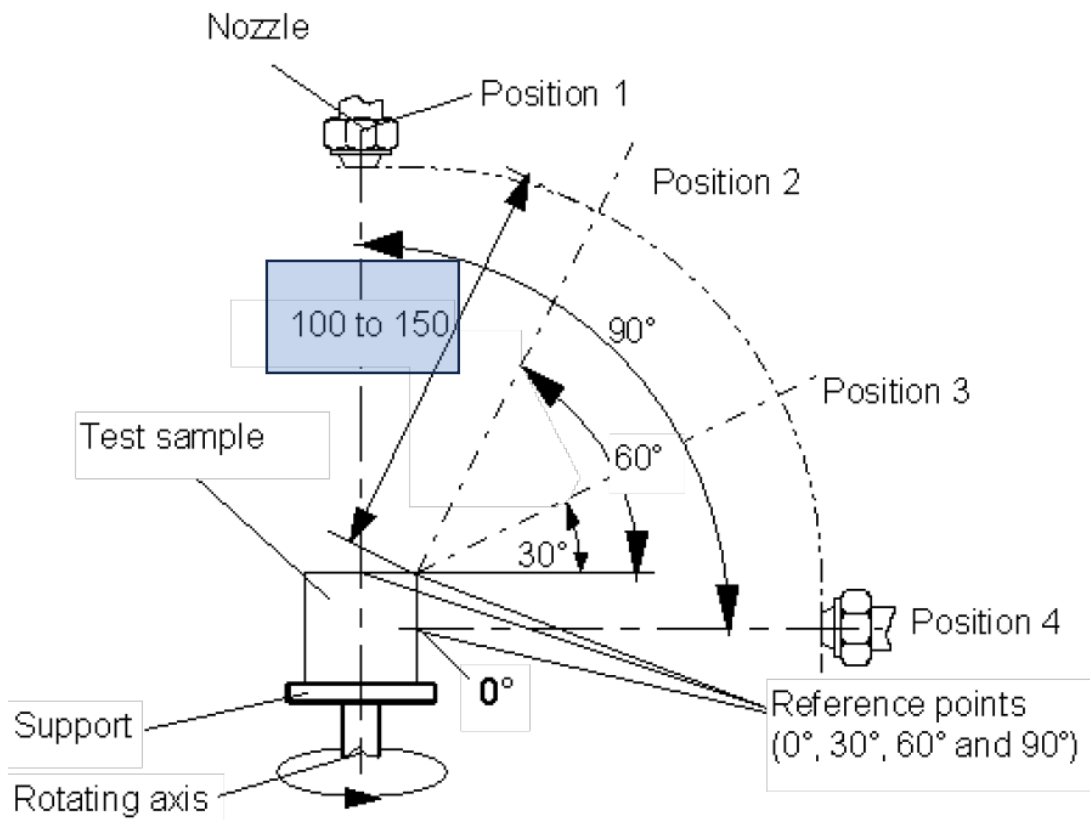
FIGURE 5.6.7.3-1: SPRAY NOZZLE AND TABLE ARRANGEMENT
