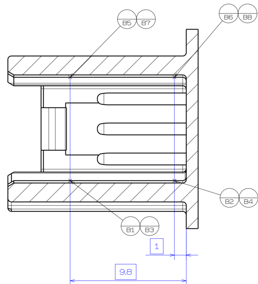
SECTION B-B
