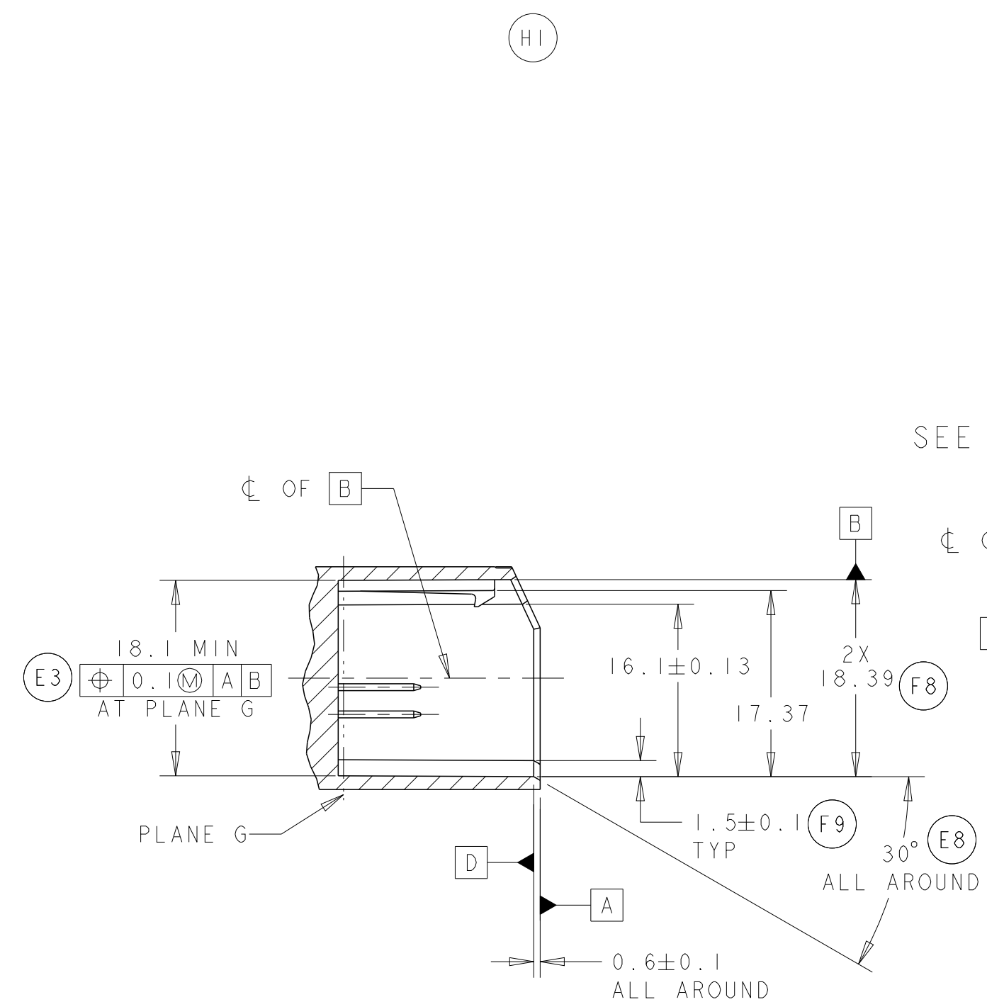
SECTION B-B
