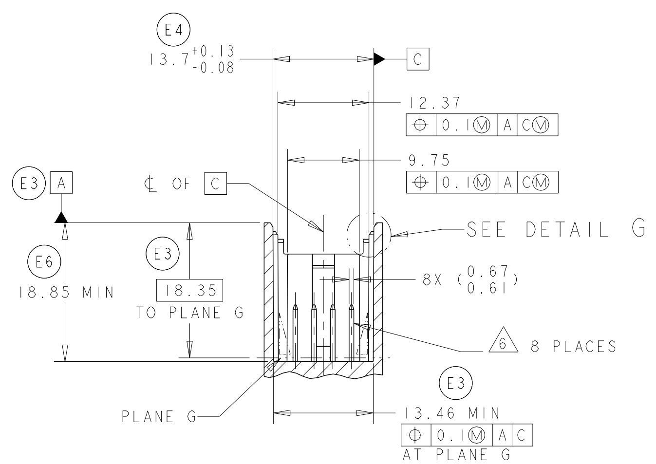
SECTION C-C
