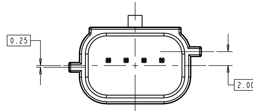
064-S-004-1-C02 (OPTION C)
