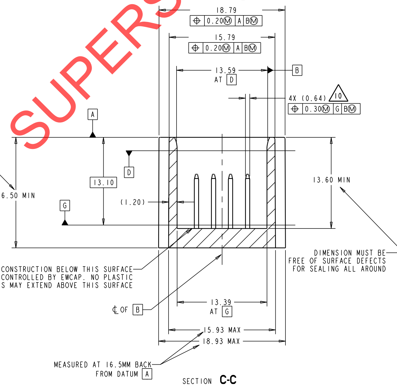
SECTION C-C
