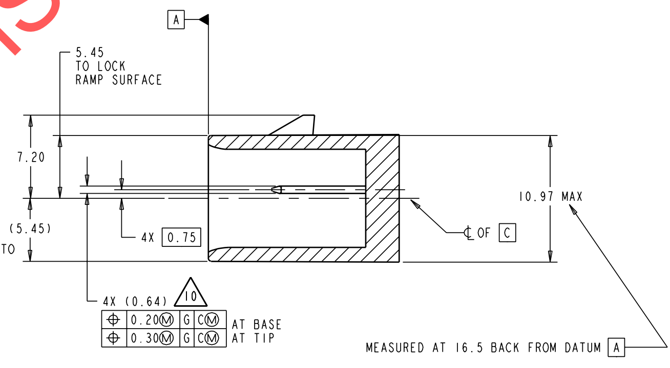
SECTION B-B
