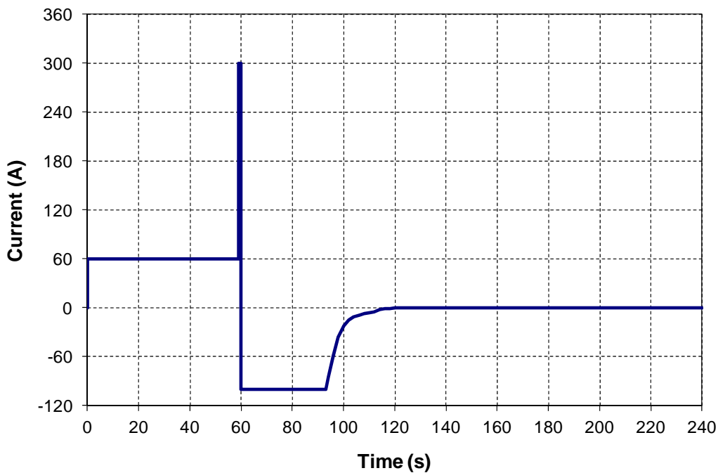
Figure 6. 12 Volt Start/Stop Cycle Life Test Profile.
