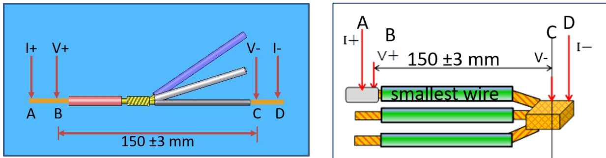
FIGURE 9 - MEASUREMENT POINTS FOR FACE-TO-FACE (LEFT) AND BUTT SPLICE (RIGHT)
