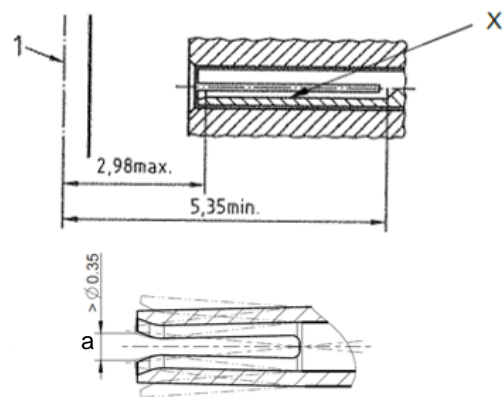
Figure 3Y - Female Contact
