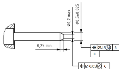
Figure 2X - Pin Dimensions
