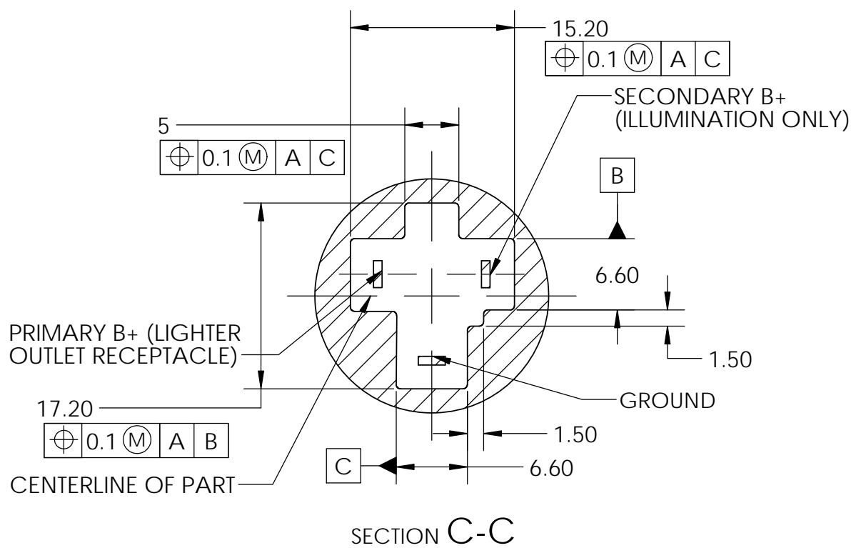
SECTION C-C
